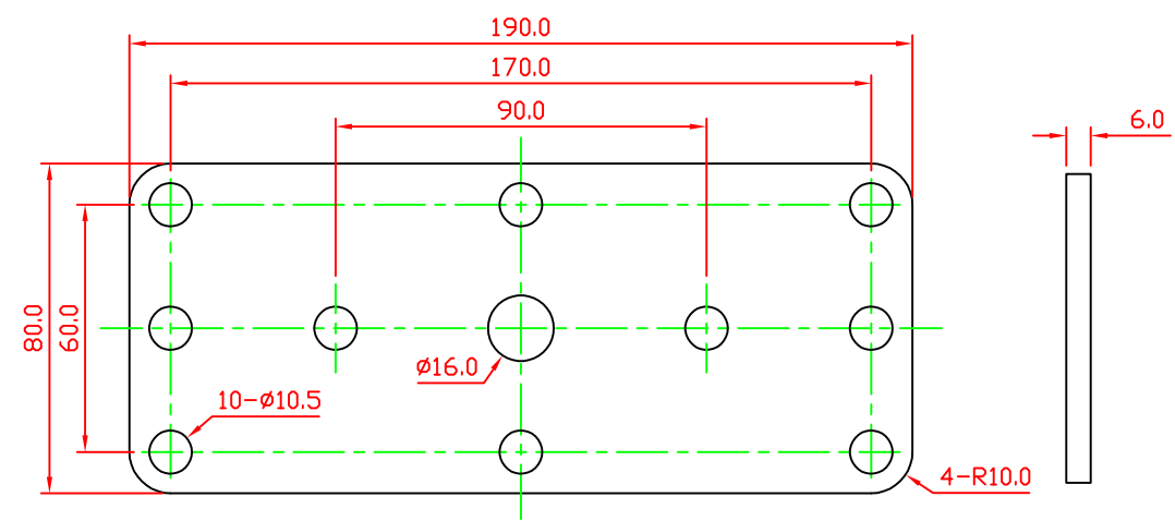
Installation plate
