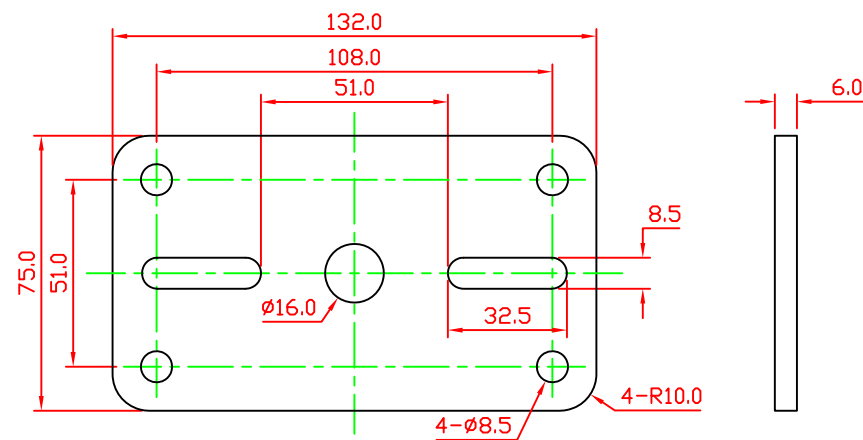
Mounting plate
