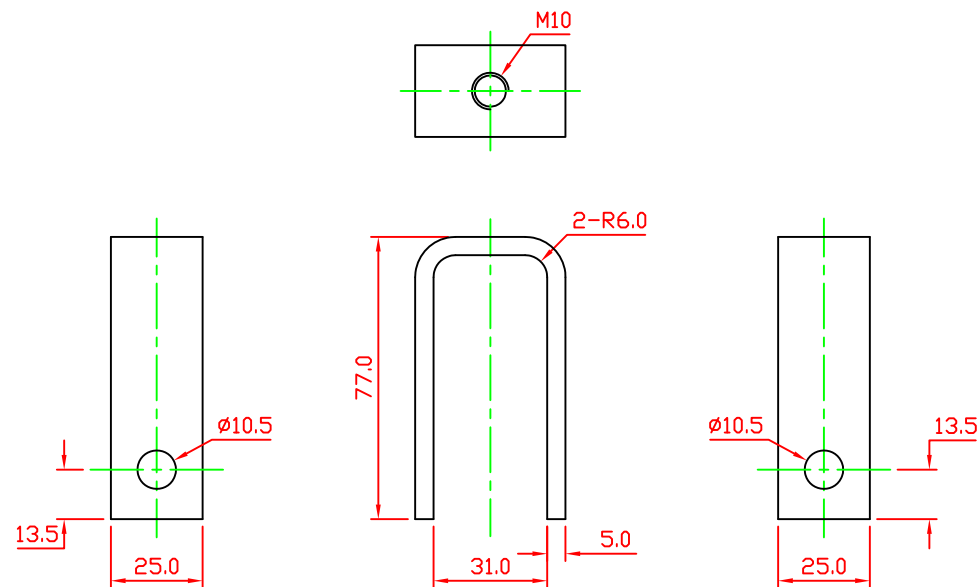
U Bracket
