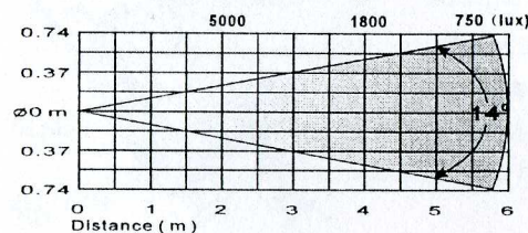
IR-6S/6B/6S/6B Beam angle: 14 degree
