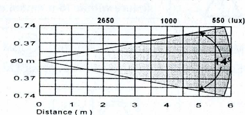
IR-6SD/IR-6BD(CDM LAMP) Beam angle: 14 degree
