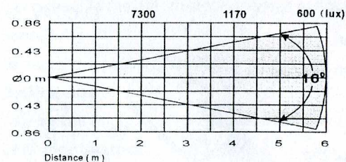
IR-4C Beam angle: 16 degree
