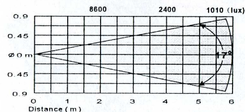
IR-5C Beam angle: 17 degree
