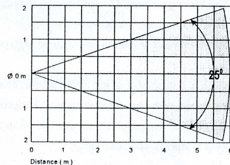
IS-4/IS-3 Beam angle: 25 degree
