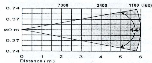
IR-7S/7B Beam angle: 14 degree
